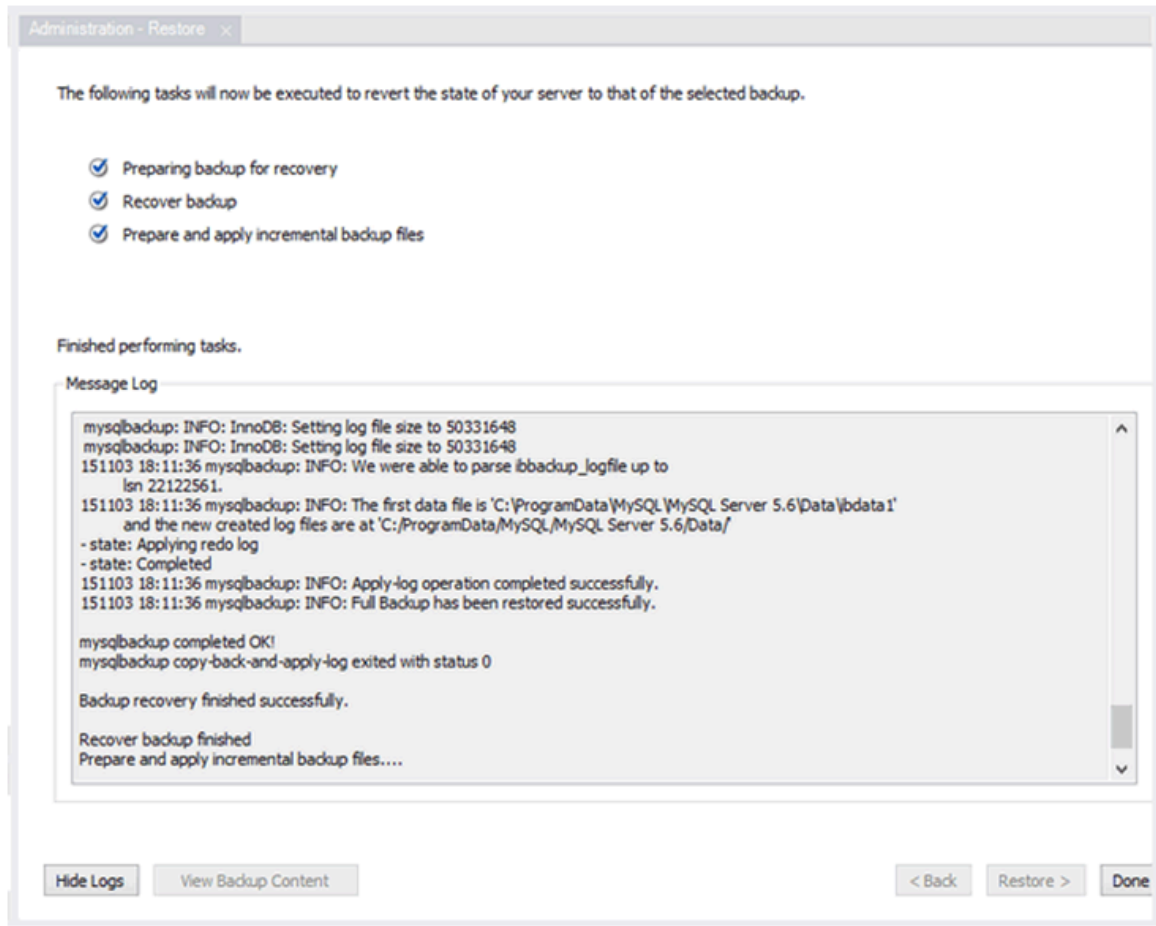
Figure 6.32 Workbench: MySQL Enterprise Backup - Recovery Tasks
